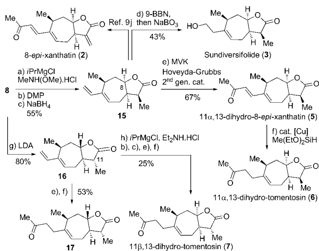
Scheme 3. Syntheses of various xanthane sesquiterpenoids from 8 . Reagents and conditions: a) i PrMgCl (5.0 equiv), MeNH(OMe)·HCl (2.5 equiv), THF, 0°C; b) DMP (1.2 equiv), CH 2 Cl 2 , RT; c) NaBH 4 (2.5 equiv), MeOH, 0°C; d) 9-BBN (5.0 equiv), THF, reflux, then NaBO 3 , RT; e) MVK (20.0 equiv), Hoveyda–Grubbs 2 nd generation cat. (10 mol%), CH 2 Cl 2 , 40°C; f) Cu(OAc) 2 (0.5 equiv), P(O i Pr) 3 (1.0 equiv), Me(EtO) 2 SiH (1.5 equiv), toluene, RT; g) LDA (5.0 equiv), THF, 0°C; h) i PrMgCl (5.0 equiv), Et 2 NH·HCl (2.5 equiv), THF, 0°C. DMP = Dess–Martin periodinane, LDA = lithium diisopropylamine, 9-BBN = 9-borabicyclo[3.3.1]nonane.
